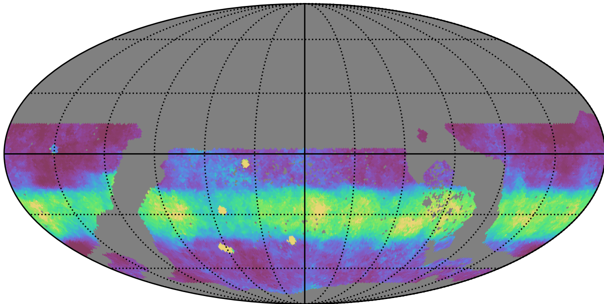
too_elab_r8_d2_giz_v3.4_10yrs WFD z band: Median normairmass
