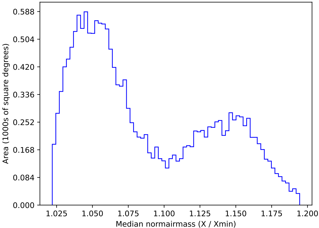
too_elab_r8_d2_giz_v3.4_10yrs WFD z band: Median normairmass
