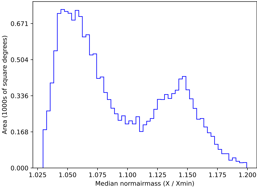
too_elab_r8_d2_giz_v3.4_10yrs WFD y band: Median normairmass
