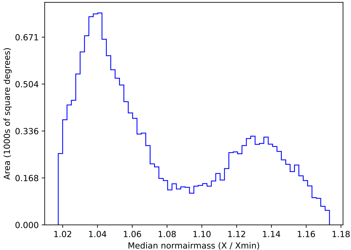
too_elab_r8_d2_giz_v3.4_10yrs WFD i band: Median normairmass
