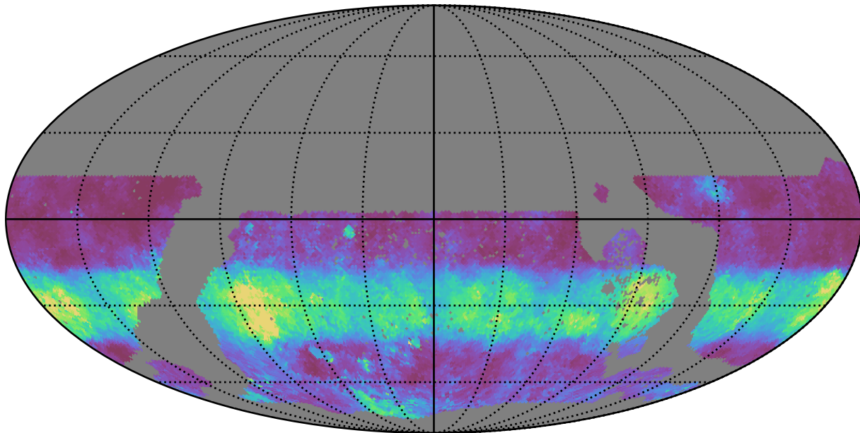
too_elab_r8_d2_giz_v3.4_10yrs WFD g band: Median normairmass
