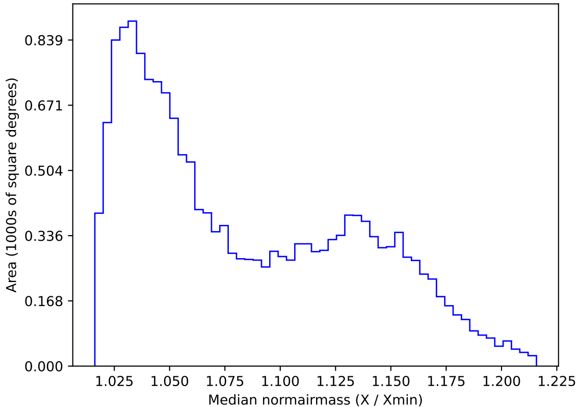
too_elab_r8_d2_giz_v3.4_10yrs WFD g band: Median normairmass
