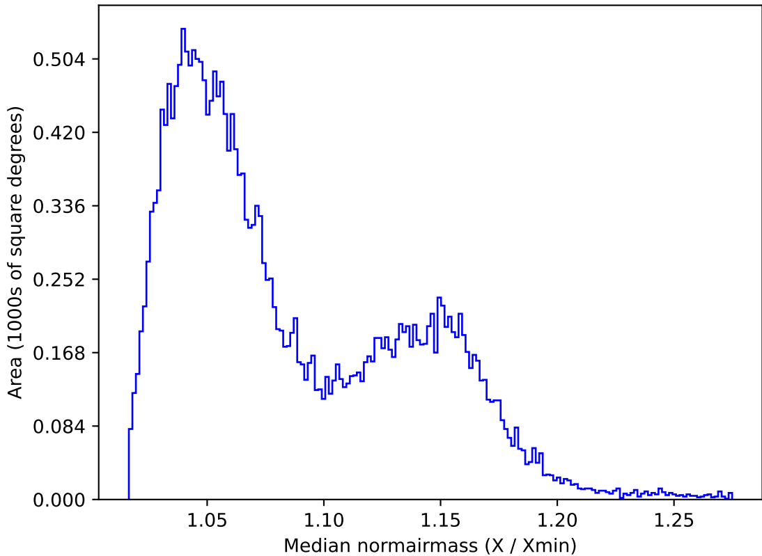
too_elab_r8_d2_giz_v3.4_10yrs All sky z band: Median normairmass
