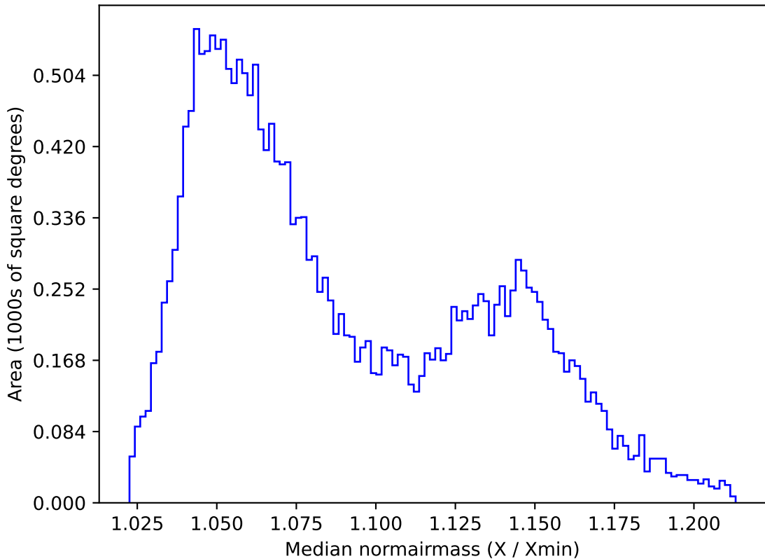
too_elab_r8_d2_giz_v3.4_10yrs All sky y band: Median normairmass
