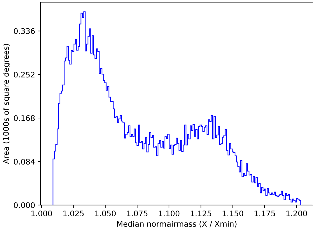
too_elab_r8_d2_giz_v3.4_10yrs All sky u band: Median normairmass
