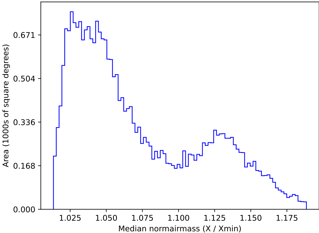
too_elab_r8_d2_giz_v3.4_10yrs All sky r band: Median normairmass
