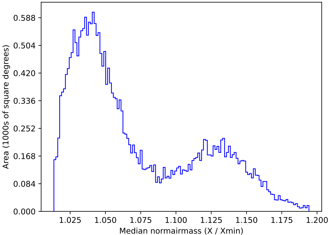
too_elab_r8_d2_giz_v3.4_10yrs All sky r band: Median normairmass
