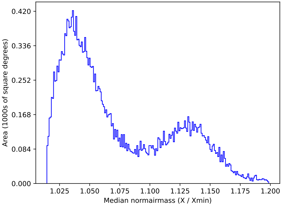
too_elab_r8_d2_giz_v3.4_10yrs All sky i band: Median normairmass
