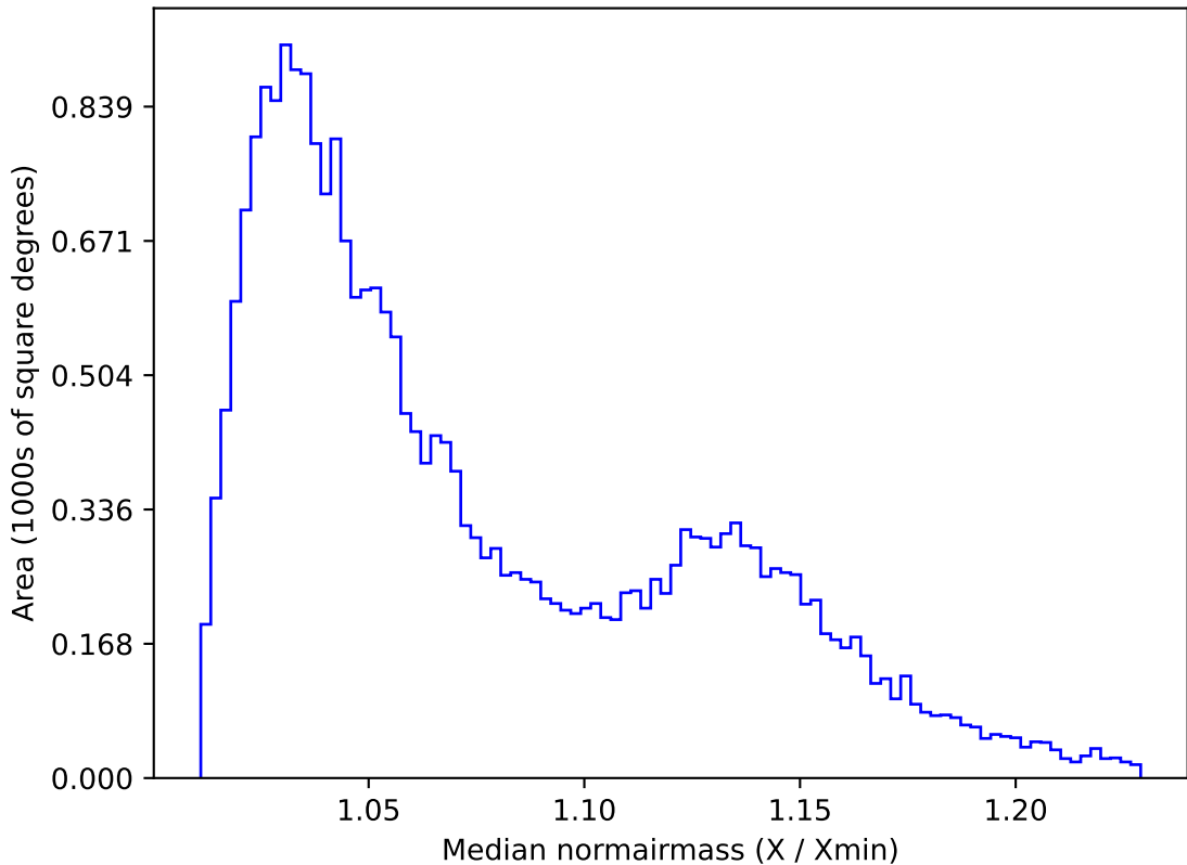
too_elab_r8_d2_giz_v3.4_10yrs All sky g band: Median normairmass
