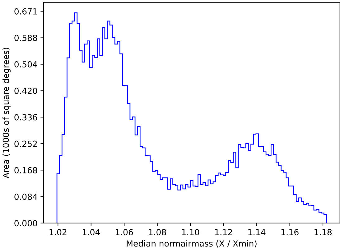
too_elab_r8_d2_giz_v3.4_10yrs All sky all bands: Median normairmass
