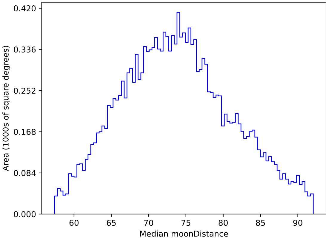
too_elab_r8_d2_giz_v3.4_10yrs WFD z band: Median moonDistance
