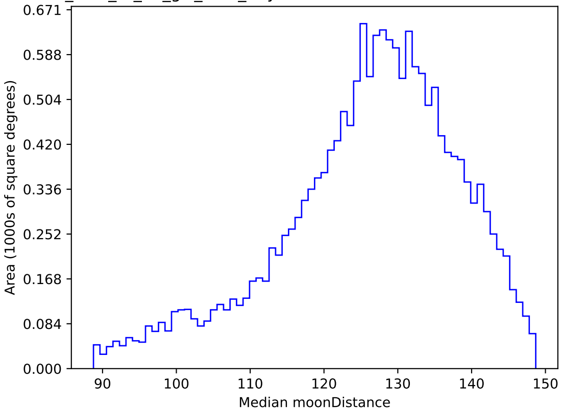
too_elab_r8_d2_giz_v3.4_10yrs WFD u band: Median moonDistance
