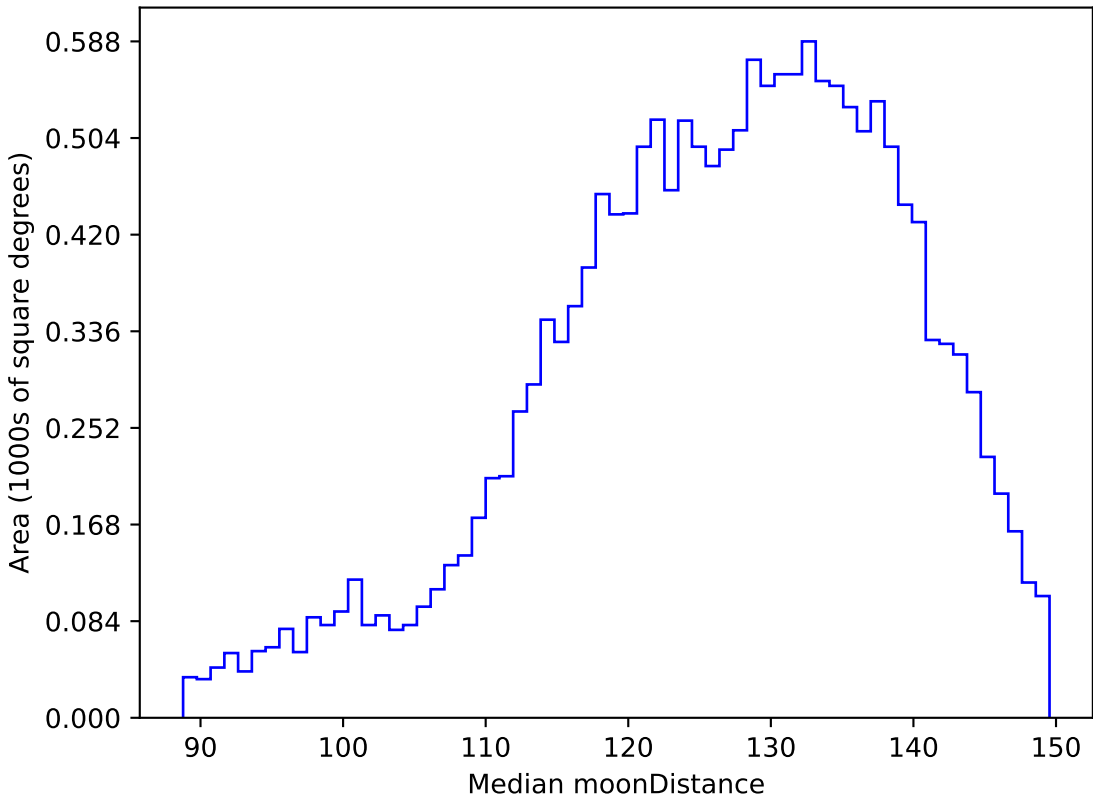
too_elab_r8_d2_giz_v3.4_10yrs WFD u band: Median moonDistance
