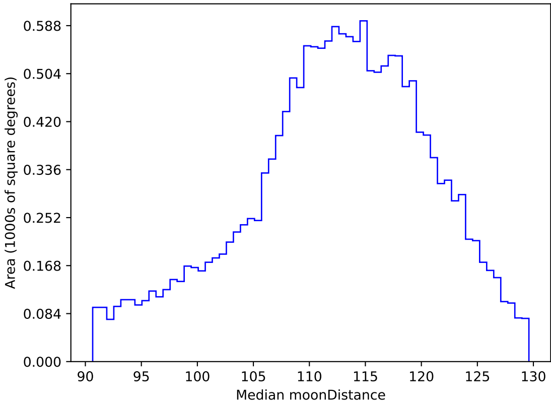
too_elab_r8_d2_giz_v3.4_10yrs WFD r band: Median moonDistance
