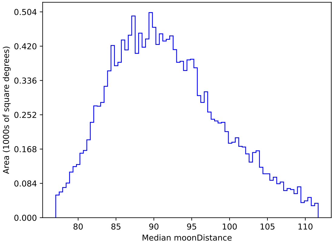
too_elab_r8_d2_giz_v3.4_10yrs WFD i band: Median moonDistance
