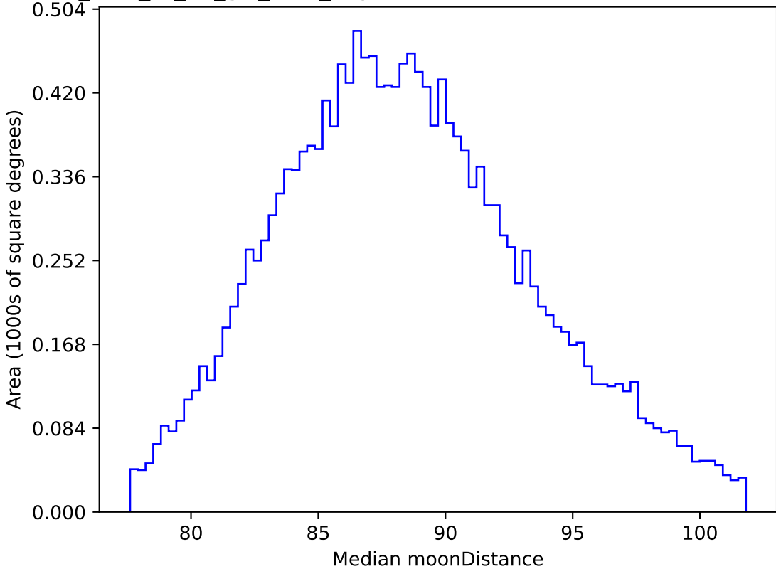
too_elab_r8_d2_giz_v3.4_10yrs WFD all bands: Median moonDistance
