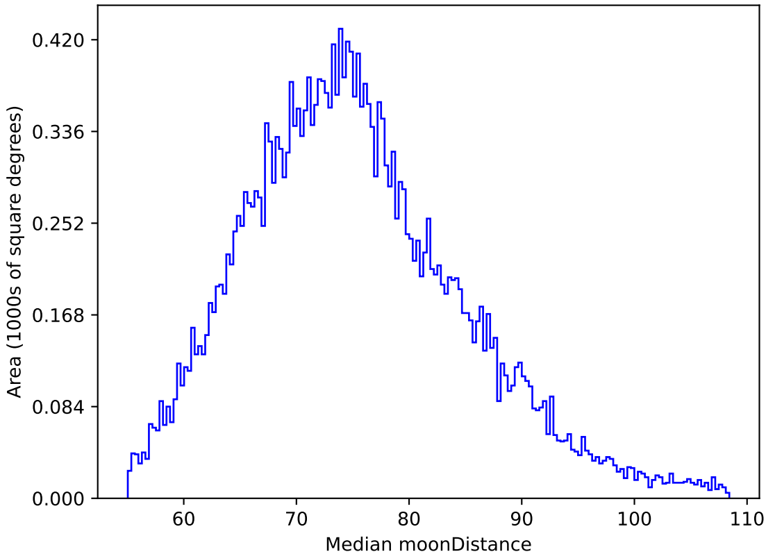
too_elab_r8_d2_giz_v3.4_10yrs All sky z band: Median moonDistance
