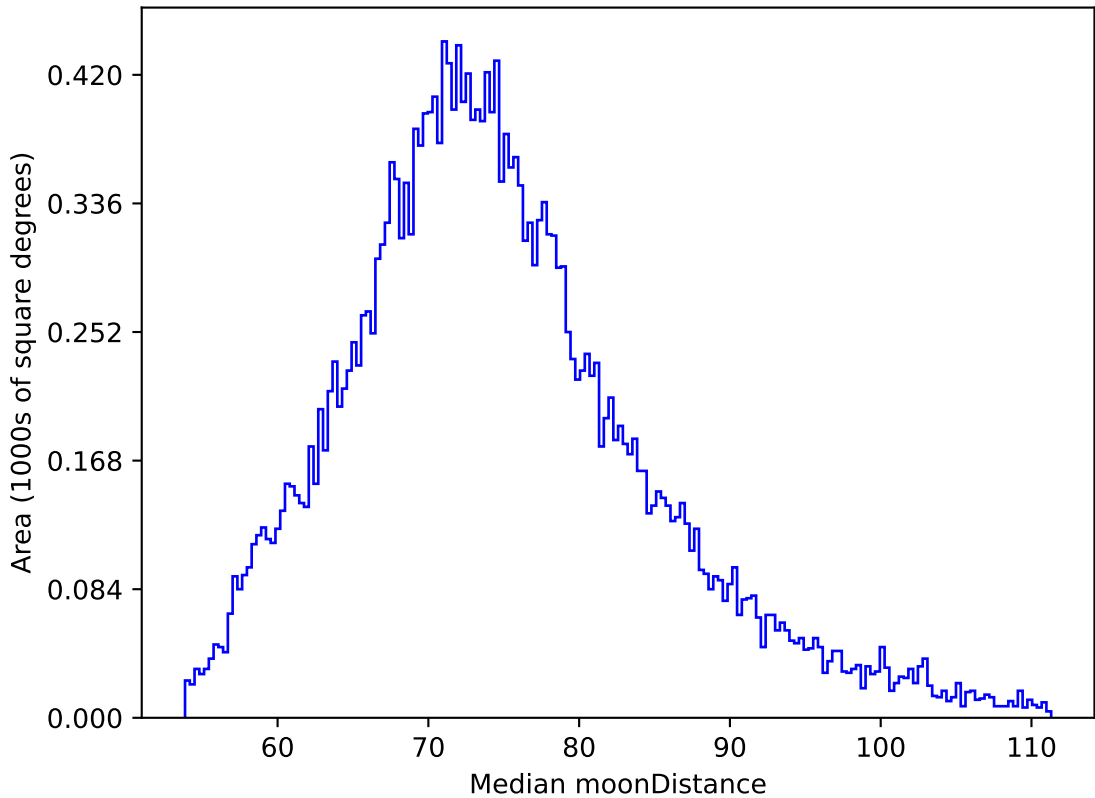
too_elab_r8_d2_giz_v3.4_10yrs All sky z band: Median moonDistance
