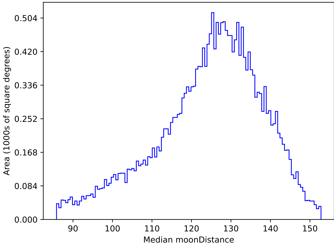
too_elab_r8_d2_giz_v3.4_10yrs All sky u band: Median moonDistance
