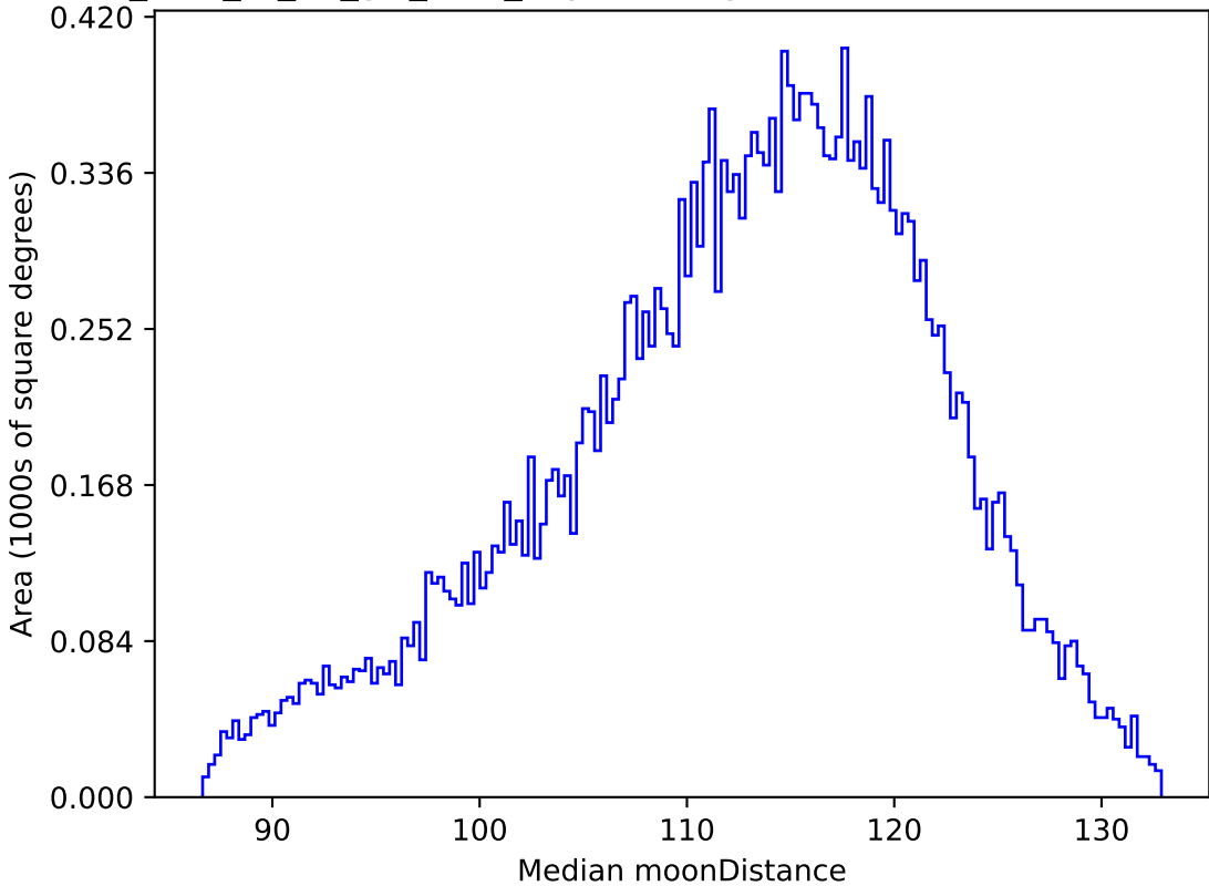
too_elab_r8_d2_giz_v3.4_10yrs All sky r band: Median moonDistance
