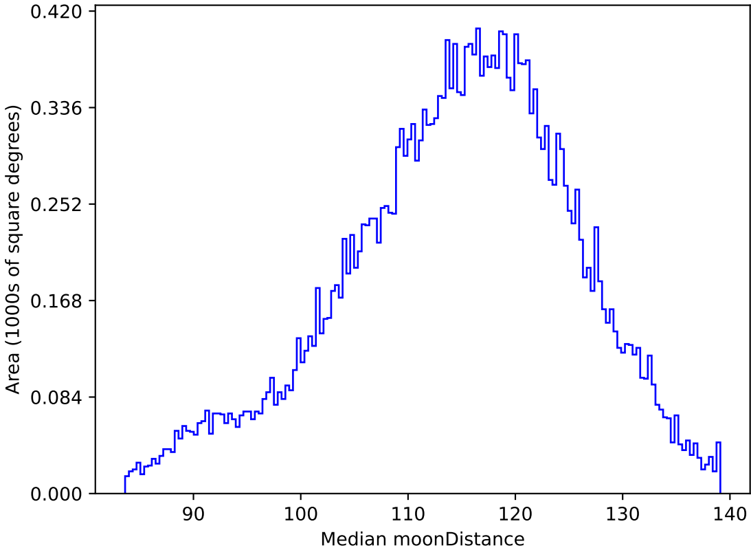
too_elab_r8_d2_giz_v3.4_10yrs All sky g band: Median moonDistance
