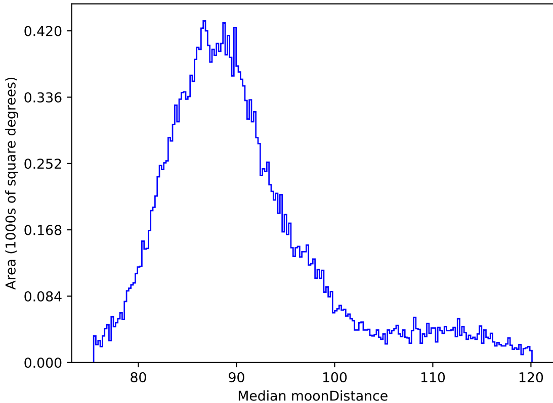
too_elab_r8_d2_giz_v3.4_10yrs All sky all bands: Median moonDistance
