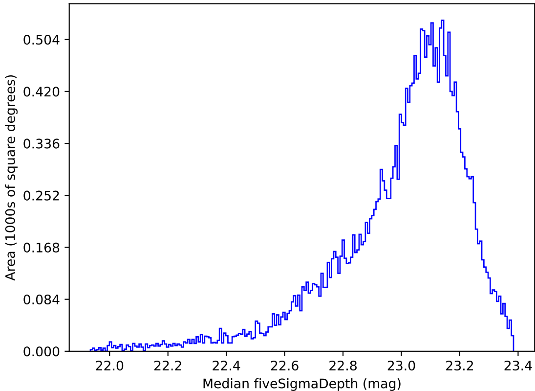
too_elab_r8_d2_giz_v3.4_10yrs Yr 1 z band: Median fiveSigmaDepth
