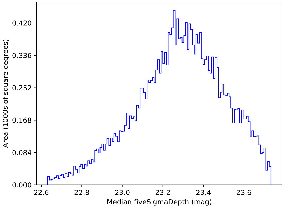
too_elab_r8_d2_giz_v3.4_10yrs Yr 1 u band: Median fiveSigmaDepth
