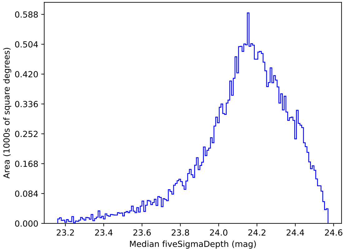
too_elab_r8_d2_giz_v3.4_10yrs Yr 1 r band: Median fiveSigmaDepth
