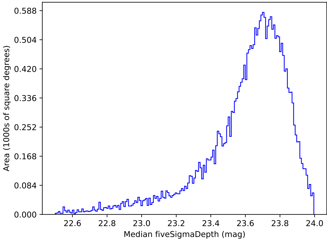
too_elab_r8_d2_giz_v3.4_10yrs Yr 1 i band: Median fiveSigmaDepth
