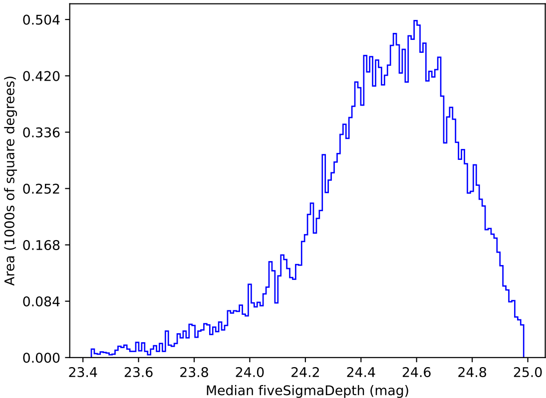
too_elab_r8_d2_giz_v3.4_10yrs Yr 1 g band: Median fiveSigmaDepth
