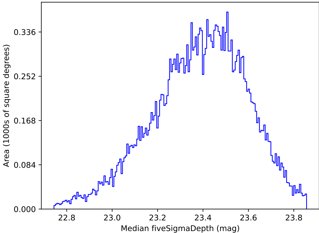
too_elab_r8_d2_giz_v3.4_10yrs Yr 1 all bands: Median fiveSigmaDepth
