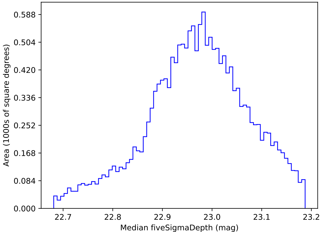
too_elab_r8_d2_giz_v3.4_10yrs WFD z band: Median fiveSigmaDepth
