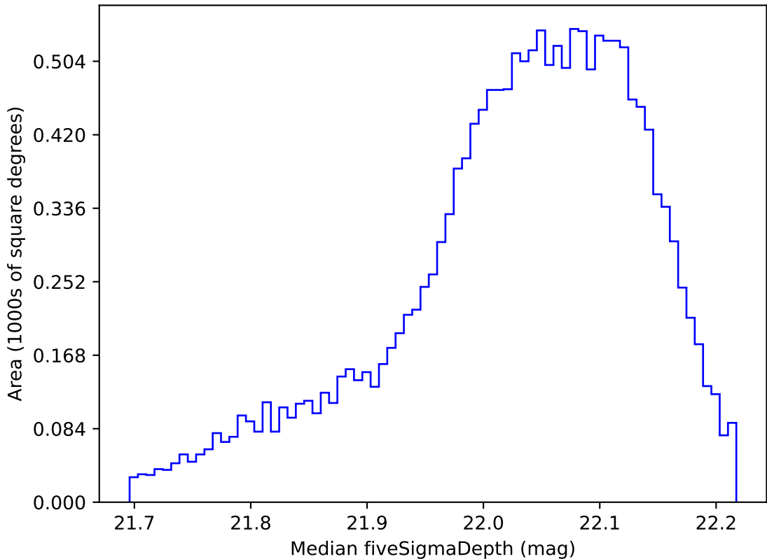
too_elab_r8_d2_giz_v3.4_10yrs WFD y band: Median fiveSigmaDepth
