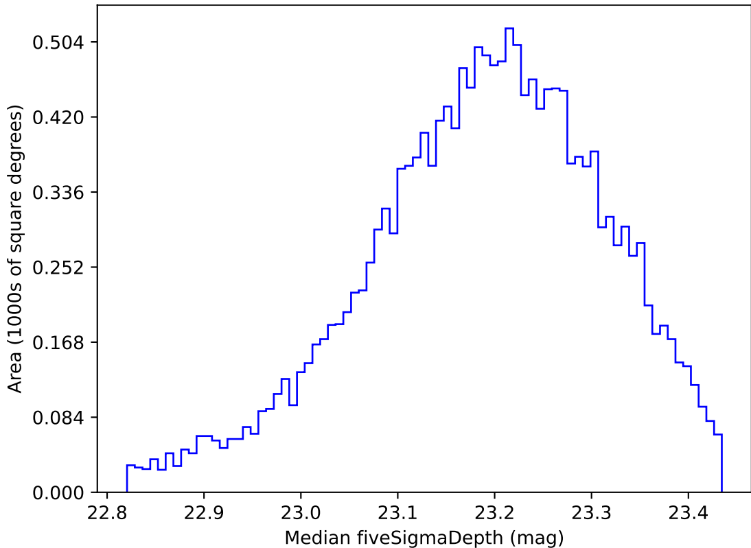
too_elab_r8_d2_giz_v3.4_10yrs WFD u band: Median fiveSigmaDepth
