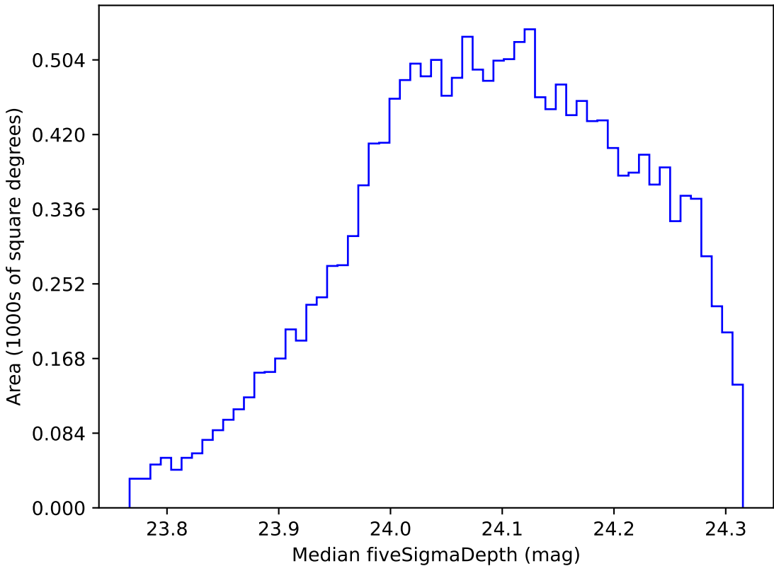
too_elab_r8_d2_giz_v3.4_10yrs WFD r band: Median fiveSigmaDepth
