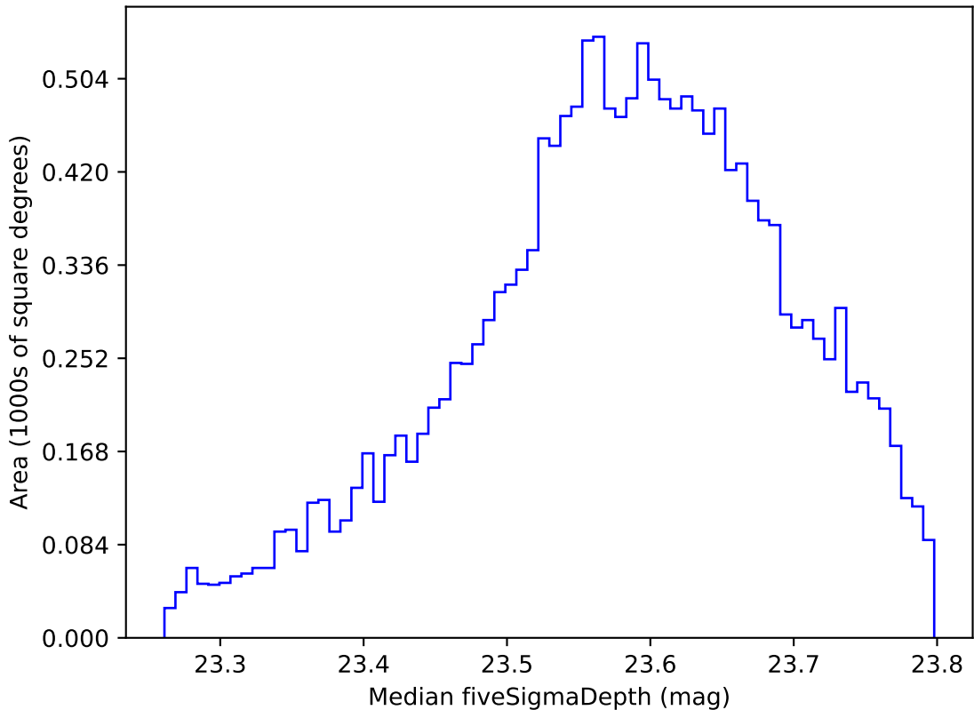
too_elab_r8_d2_giz_v3.4_10yrs WFD i band: Median fiveSigmaDepth
