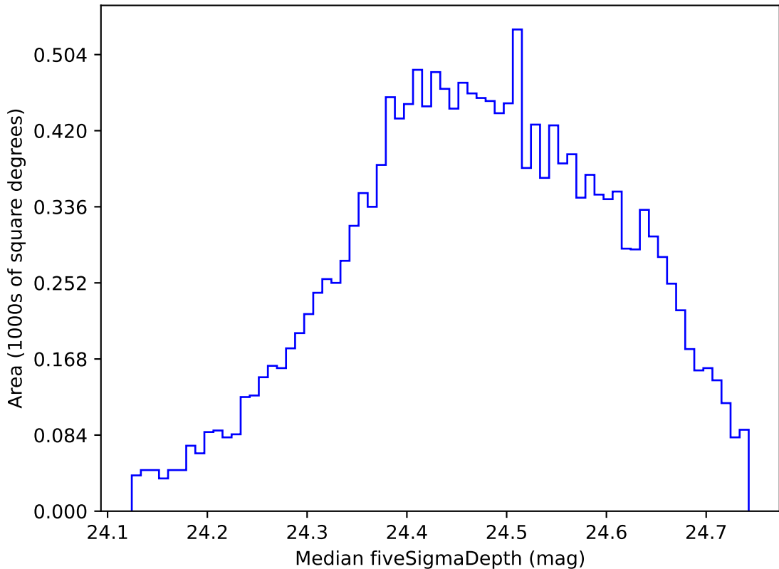
too_elab_r8_d2_giz_v3.4_10yrs WFD g band: Median fiveSigmaDepth
