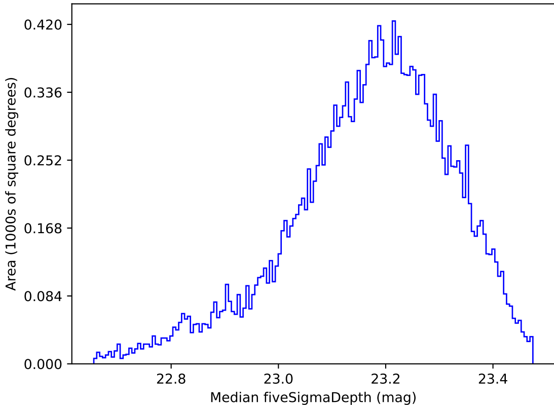
too_elab_r8_d2_giz_v3.4_10yrs All sky u band: Median fiveSigmaDepth
