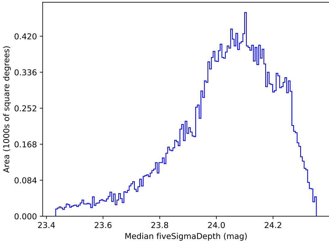
too_elab_r8_d2_giz_v3.4_10yrs All sky r band: Median fiveSigmaDepth
