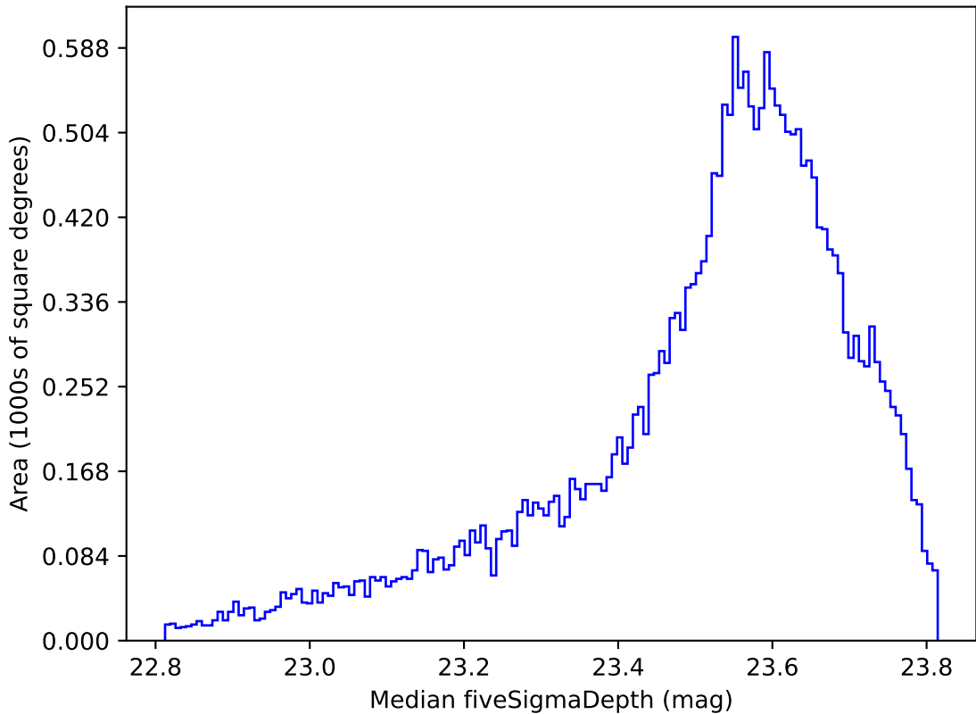
too_elab_r8_d2_giz_v3.4_10yrs All sky i band: Median fiveSigmaDepth
