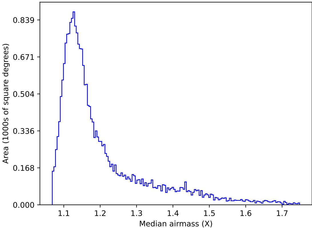
too_elab_r8_d2_giz_v3.4_10yrs Yr 1 y band: Median airmass
