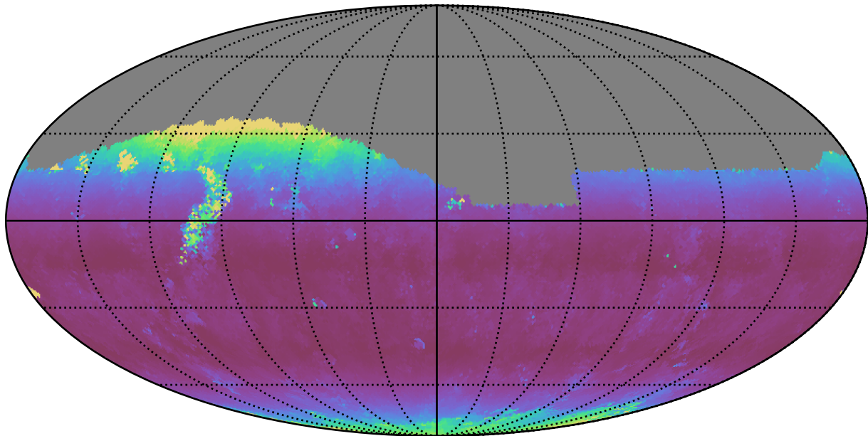
too_elab_r8_d2_giz_v3.4_10yrs Yr 1 i band: Median airmass
