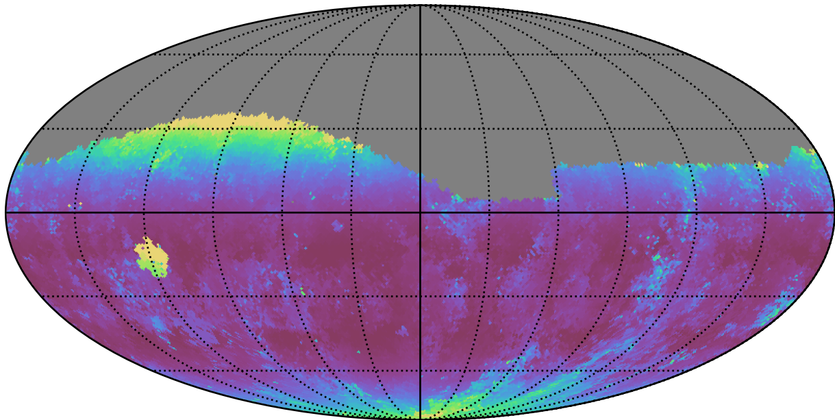
too_elab_r8_d2_giz_v3.4_10yrs Yr 1 g band: Median airmass
