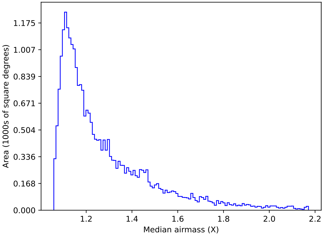
too_elab_r8_d2_giz_v3.4_10yrs Yr 1 g band: Median airmass
