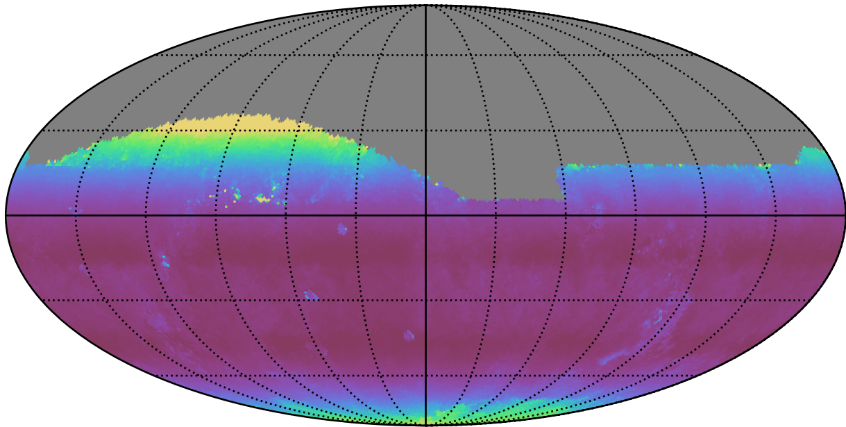
too_elab_r8_d2_giz_v3.4_10yrs Yr 1 all bands: Median airmass
