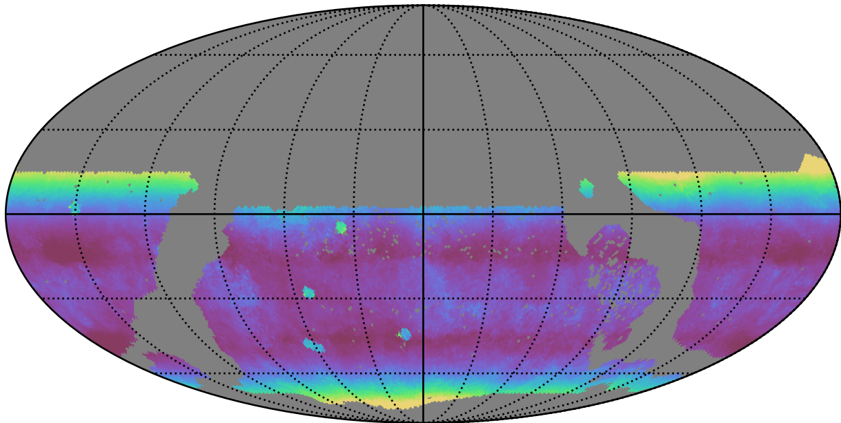
too_elab_r8_d2_giz_v3.4_10yrs WFD z band: Median airmass
