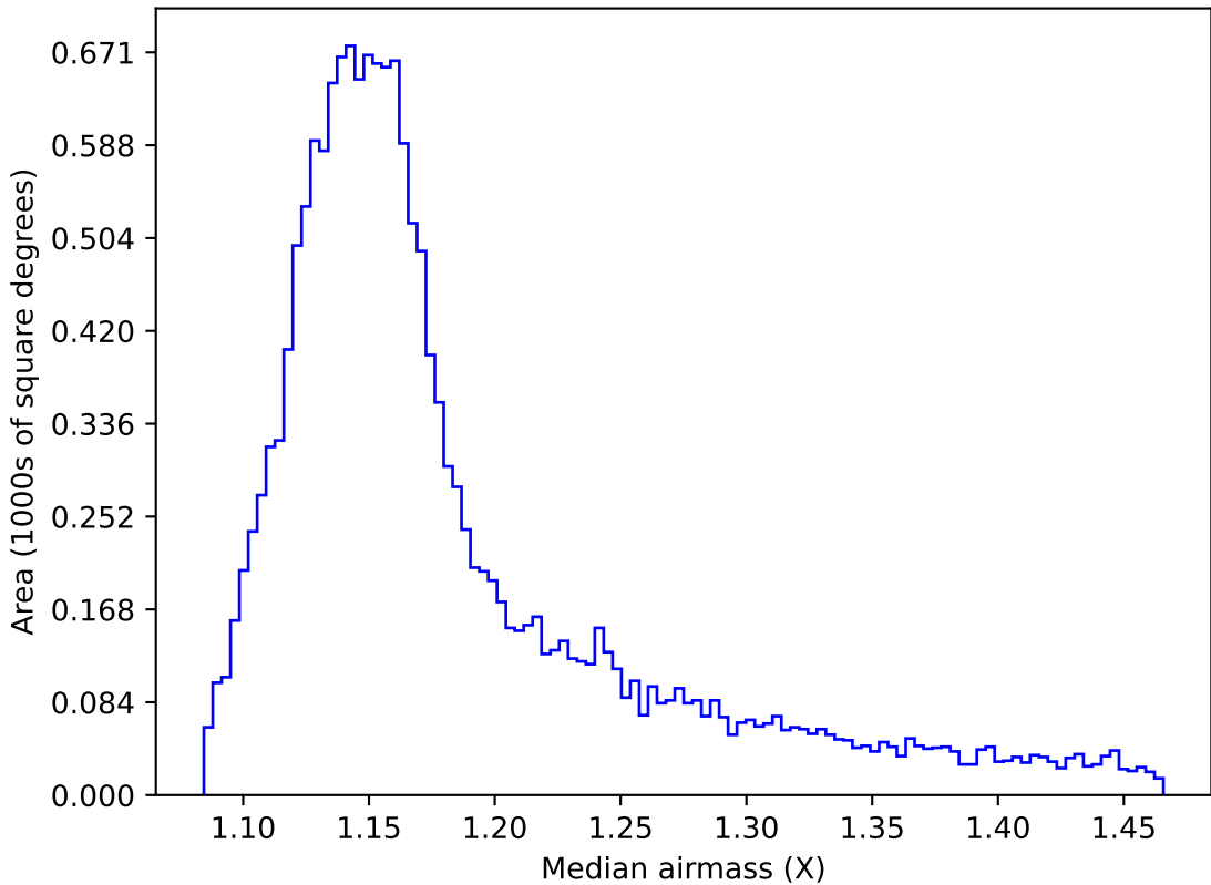
too_elab_r8_d2_giz_v3.4_10yrs WFD z band: Median airmass
