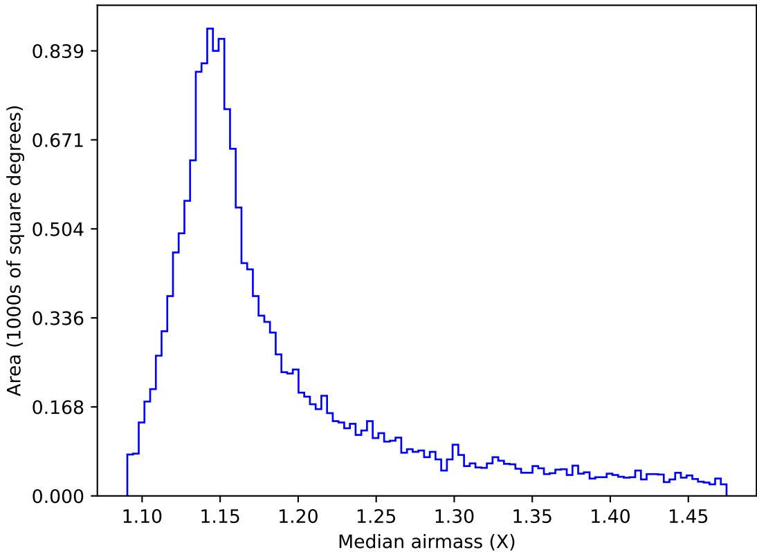
too_elab_r8_d2_giz_v3.4_10yrs WFD y band: Median airmass
