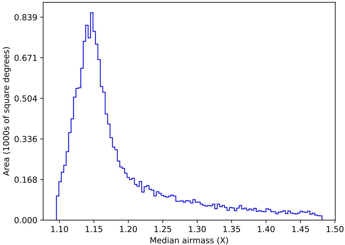
too_elab_r8_d2_giz_v3.4_10yrs WFD y band: Median airmass
