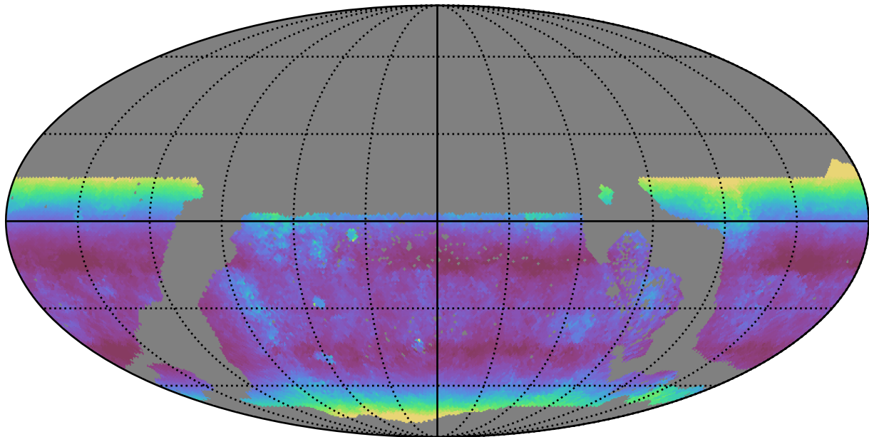
too_elab_r8_d2_giz_v3.4_10yrs WFD u band: Median airmass
