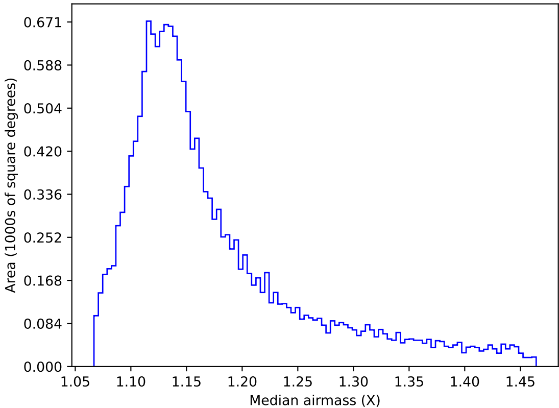
too_elab_r8_d2_giz_v3.4_10yrs WFD u band: Median airmass
