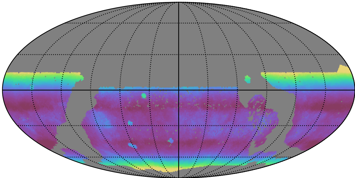
too_elab_r8_d2_giz_v3.4_10yrs WFD r band: Median airmass
