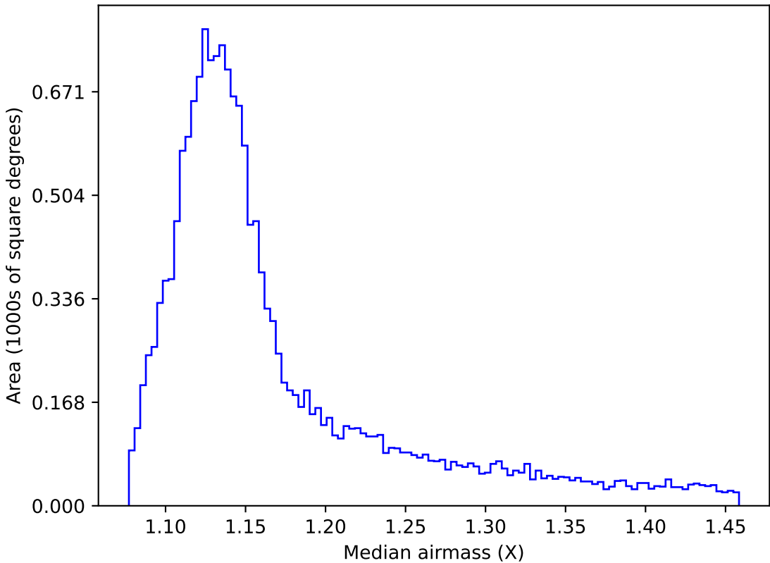
too_elab_r8_d2_giz_v3.4_10yrs WFD i band: Median airmass
